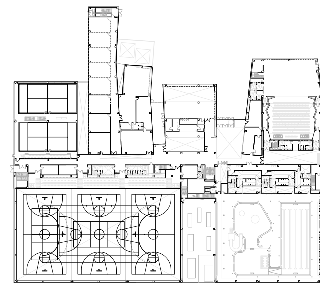
MAIN FLOOR
