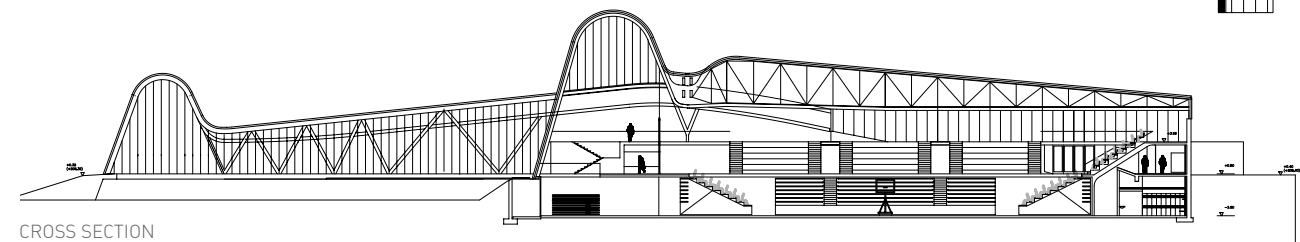
CROSS SECTION
