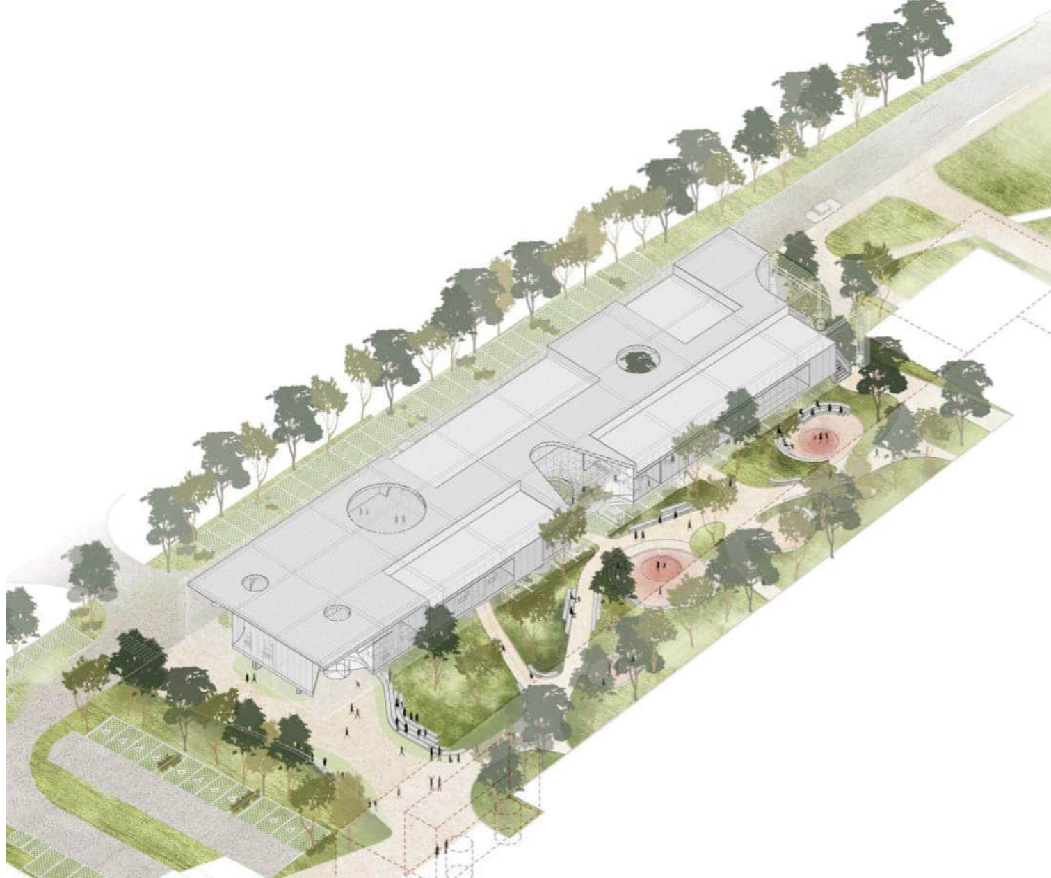
Modified views with microtopography and vegetation
